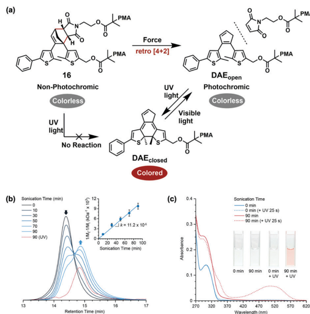
Fig. 18 (a) Mechanochemically gated photoswitching using a cyclopentadiene–maleimide mechanophore. (b) GPC traces (RI) and molecular weight data for polymer 16 before and after ultrasonication time. (c) UV-vis absorption spectra of polymer 16 before and after ultrasonication and UV irradiation demonstrating mechanochemically gated photoswitching. Reproduced with permission. 58 Copyright 2018, American Chemical Society.
