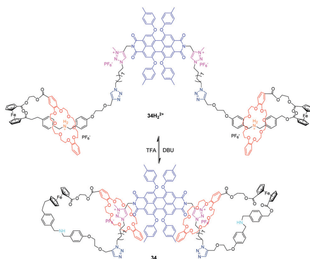
Fig. 34 pH-Controllable bis[1]rotaxane 34 .
