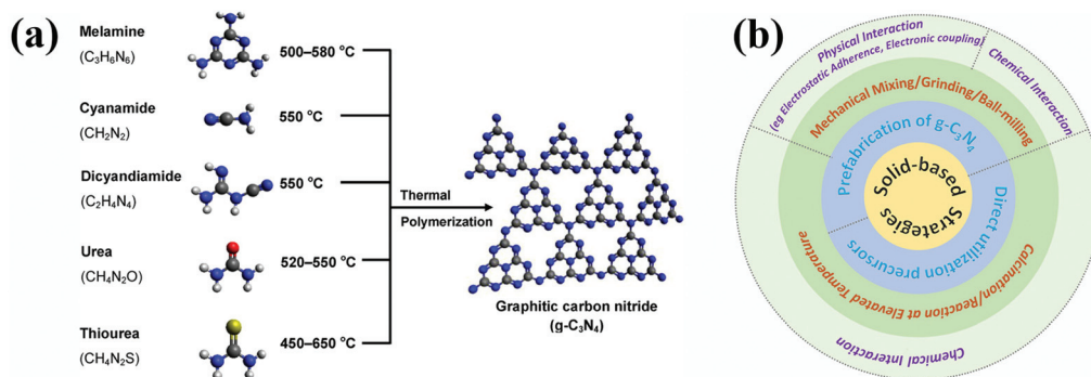
Fig. 2 (a) Graphical illustration of the general preparation conditions for g\text{-C}_3\text{N}_4 from various organic precursors, where the blue, grey, white, red and yellow balls represent N, C, H, O, S atoms, respectively. Reproduced from ref. 41 with permission from the American Chemical Society, Copyright 2016. (b) Synthetic strategies for g\text{-C}_3\text{N}_4 composite photocatalysts with interface contacts based on solid-state conditions.
