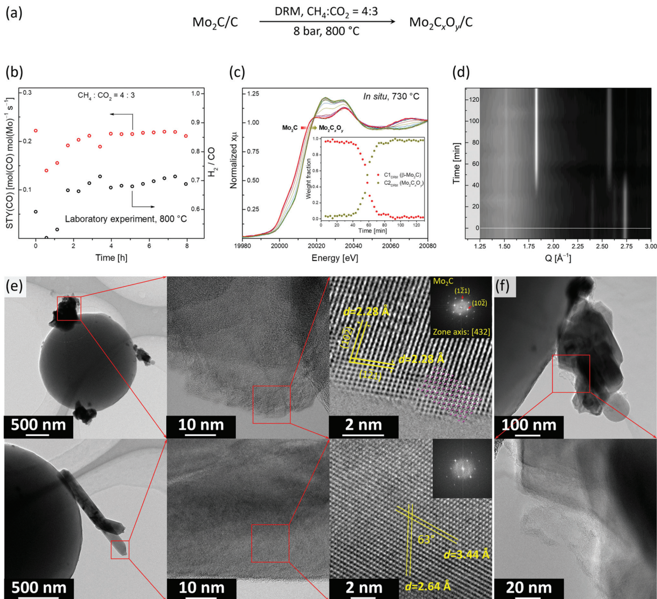
Fig. 3 (a) Schematic of the experimental conditions during the DRM experiment; (b) catalytic performance of β-Mo 2 C/C in DRM (laboratory scale reactor, 800 °C, 8 bar, SV = 550 L g Mo -1 h -1 ); DRM experiment followed by (c) Mo K-edge XANES, where the inset shows the phase evolution according to MCR-ALS, and (d) XRD (Q = 4π sin(θ)/λ) (capillary reactor, 730 °C, 8 bar, SV = 3500 L g Mo -1 h -1 ); (e) TEM and HR-TEM images of the spent Mo 2 C x O y /C catalyst revealing two different morphologies, i.e. aggregates of nanoplates (top) and nanorods (bottom); (f) TEM images of amorphous carbon deposited on the active Mo 2 C x O y /C catalyst.
