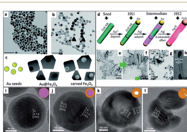
Fig. 9 Hollow nanostructures derived from HNSs. (a–c) Au NPs serve as seeds for the growth of a shell (Au@Fe 3 O 4 , TEM shown in (a)), subsequently etched with iodine, removing the gold and resulting in carved Fe 3 O 4 (b); scale bars are 100 nm; (c) scheme. 130 (d–h) The nanoscale Kirkendall effect is responsible for the formation of Ag 2 S nanotubes with a gold–silver tip: (d) the synthetic scheme, (e) ZnS NRs ( d ~ 3 nm) serve as seeds for the reduction of gold on its tips (HS1, shown in (f)); following the exposure of HS1 to Ag + ions two phenomena occur—the Au tip is alloyed to form an AuAg tip and the rod is transformed via the Kirkendall effect (silver cations diffuse inside, replacing the zinc cations, which diffuse outside) resulting in a hollow silver sulfide nanotube, Ag 2 S NT/AuAg (HS2); confirmation of the mechanism is evident from TEM images (g), where d ~ 5 nm; a wall thickness of 0.8 ± 0.1 nm is confirmed by (h) HRTEM. 243 (i–l) Hollow indium oxide NPs are formed via a non-Kirkendall mechanism in a deaerated atmosphere, 249 namely In NPs (i) with a native amorphous InO x shell are first thermally oxidized to form an In@In 2 O 3 core@shell (j), additional heating is responsible for crack formation due to thermal expansion and void-formation, resulting in hollow In 2 O 3 (k); some NPs exhibit significant cracking shown in (l); the inset of every TEM image contains a schematic cartoon of the NS. (a–c) Adapted from ref. 130 with permission from the Royal Society of Chemistry, copyright 2018. (d–h) Adapted from ref. 243 with permission from the Royal Society of Chemistry, copyright 2015. (i–l) Adapted with permission from Wiley-VCH Verlag GmbH & Co., copyright 2013.
