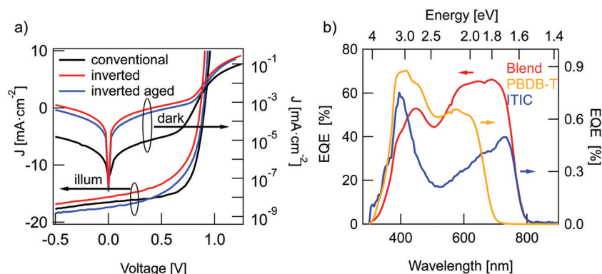
Fig. 2 Solar cell characteristics. (a) J-V -curves of PBDB-T:ITIC solar cells in dark and under illumination: conventional (black traces), inverted (red) and aged inverted (blue). (b) EQE spectra for inverted solar cells (red trace) together with diodes from pure PBDB-T (yellow) and pure ITIC (blue).
