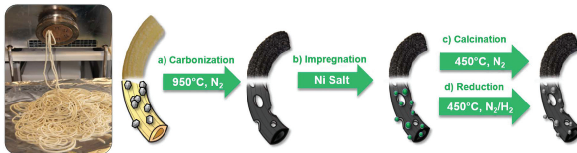
Fig. 3 Schematic representation of the catalyst synthesis protocol starting from the extrusion, carbonization, calcination, and reduction steps.
