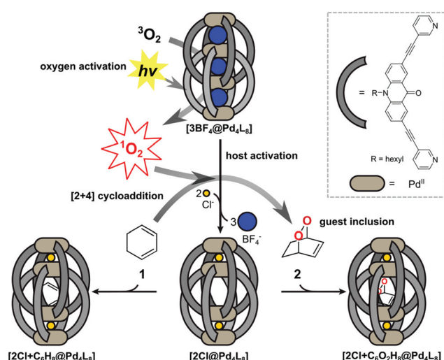
Fig. 1 Catalytic function and guest inclusion behaviour of the acridone-based double cages [3\text{BF}_4\text{Pd}_4\text{L}_8] and [2\text{Cl}@Pd_4\text{L}_8] : both cages are able to generate singlet oxygen, reacting in a [2+4] cycloaddition reaction with 1,3-cyclohexadiene. Only [2\text{Cl}@Pd_4\text{L}_8] is able to encapsulate both substrate 1 and product 2 .
