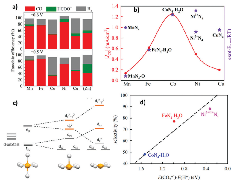
Fig. 20 (a) FE at -0.6 V (up) and -0.5 V (bottom) vs. RHE obtained over the M-N-C catalysts (M = Mn, Fe, Co, Ni, and Cu) for 90 min electrolysis under CO_2 -saturated 0.1 M KHCO_3 aqueous electrolyte (pH 6.7) at room temperature. (b) Comparison of experimental CO partial current density at -0.6 V vs. RHE for pyrolyzed M-N-C materials and DFT calculated trends ( U = -0.6 V vs. RHE). E_{RDS} is the calculated free reaction energy at the specific RDS of CO_2RR to CO for each active site. (c) Octahedral, square pyramid and square planar symmetry (orange indicates the antibonding states). (d) The experimental selectivity at -0.6 V vs. RHE over Fe-N-C, Co-N-C, and Ni-N-C vs. the DFT-simulated E(*CO_2^-) - E(*H) . 306 Adapted with permission from ref. 306. Copyright 2019 American Chemical Society.
