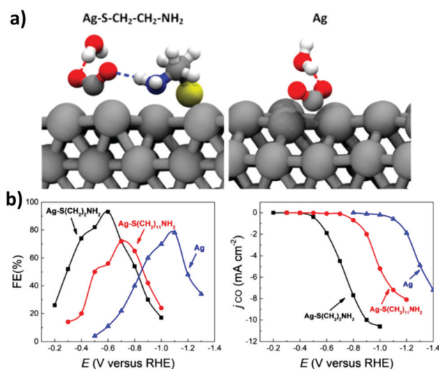
Fig. 31 (a) Chemisorbed CO 2 on cysteamine-functionalized (left) and cysteamine-free (right) Ag(111) surface. Only the water molecules directly forming hydrogen bond (slashed line) are shown. The colors are: Ag in silver, C in gray, O in red, N in blue, S in yellow, and H in white. (b) Influence of the alkyl chain length on CO 2 RR in terms of FE CO (left) or j CO (right) vs. potential. Reproduced with permission from ref. 419. Copyright 2018 American Chemical Society.
