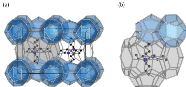
Fig. 4 (a) The structure of TBAB hydrate ((C 4 H 9 ) 4 N + Br - ·38H 2 O). The solid lines represent the unit-cell of each hydrate. (b) Magnification of TBAB hydrate structure near tetra- n -butylammonium cation. The blue shaded dodecahedral cages are empty, and as such are candidates for engaging small molecules.
