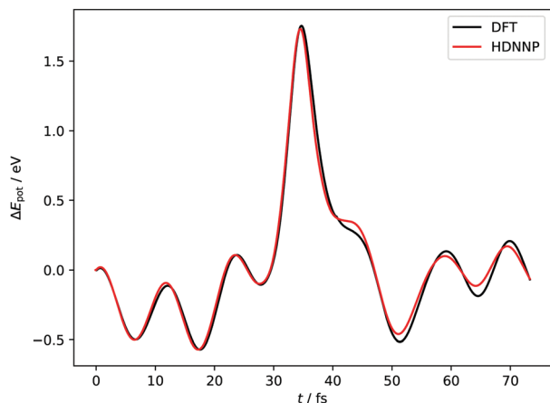
Fig. 4 Potential energies from AIMD and HDNNP trajectories with E_i = 1.9 eV, \theta_i = 34^\circ and \phi_i = 0^\circ . The two trajectories were launched with identical initial conditions and both traverse the chemisorption well before returning to the gas phase after a single bounce. The distance of closest approach is below r_{CH} = 1.4 Å. Movies of the two trajectories can be found in the ESI.†
