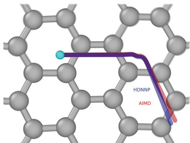
Fig. 5 The same two trajectories as in Fig. 4—AIMD (red) and HDNNP (blue). The H-atom's initial position is shown as a cyan colored ball. The divergence between the two trajectories is due to residual error in the NN fit to the DFT data. A "side view" of the trajectories can be found in the ESI.†
