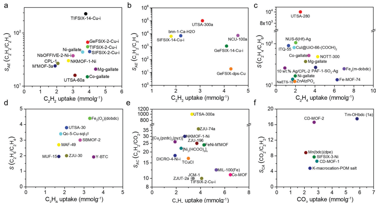
Fig. 16 Selectivity versus uptake plots for (a) \text{C}_2\text{H}_2/\text{C}_2\text{H}_4 selective adsorbents with a threshold \text{C}_2\text{H}_2 selectivity, S_{\text{AE}} > 15 (calculated for 1:99 mixtures of \text{C}_2\text{H}_2:\text{C}_2\text{H}_4 unless otherwise stated in Table 1); (b) \text{C}_2\text{H}_2/\text{C}_2\text{H}_4 selective adsorbents that exhibit molecular sieving (calculated for 1:99 mixtures of \text{C}_2\text{H}_2:\text{C}_2\text{H}_4 unless otherwise stated in Table 1). The IAST derived selectivities are therefore qualitative; (c) \text{C}_2\text{H}_4/\text{C}_2\text{H}_6 selective adsorbents with a threshold \text{C}_2\text{H}_4 selectivity, S_{\text{C}_2\text{H}_4/\text{C}_2\text{H}_6} > 10 (calculated for 1:1 mixtures of \text{C}_2\text{H}_4:\text{C}_2\text{H}_6 unless otherwise stated in Table 2); (d) \text{C}_2\text{H}_6/\text{C}_2\text{H}_4 selective adsorbents with a threshold \text{C}_2\text{H}_6 selectivity, S_{\text{C}_2\text{H}_6/\text{C}_2\text{H}_4} > 1.9 (calculated for 1:1 mixtures of \text{C}_2\text{H}_6:\text{C}_2\text{H}_4 unless otherwise stated in Table 3); (e) \text{C}_2\text{H}_2/\text{CO}_2 selective adsorbents with a threshold \text{C}_2\text{H}_2 selectivity, S_{\text{AC}} > 10 (calculated for 1:1 mixtures of \text{C}_2\text{H}_2:\text{CO}_2 unless otherwise stated in Table 4); (f) \text{CO}_2/\text{C}_2\text{H}_2 selective adsorbents (calculated for 1:1 or 2:1 mixtures of \text{CO}_2:\text{C}_2\text{H}_2 as stated in Table 4). Uptakes and selectivities are considered at 1 bar, at the temperatures specified in Tables 1–4.
