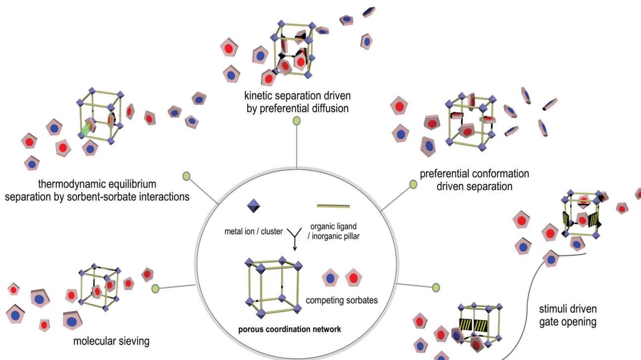
Fig. 5 There are multiple mechanisms for the adsorptive separation of C 2 LHs by PCNs as illustrated clockwise from bottom left: molecular sieving by size/shape exclusion; thermodynamic equilibrium separation; differential diffusivity driven kinetic separation; conformational preference guided separation; stimuli driven network switching based upon separation concomitant with gate opening.
