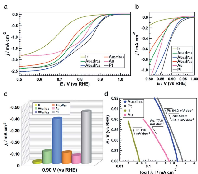
Fig. 5 Electrochemical oxygen-reduction activities of \text{Au}_x\text{Ir}_{1-x} alloy catalysts. (a), (b) rotating disk electrode l - V polarization curves taken in \text{O}_2 -saturated 1.0 M NaOH aqueous solution normalized by the glassy carbon electrode geometric area ( 0.196 \text{ cm}^2 ) from 0.50 to 1.05 \text{V}_{\text{RHE}} and (b) from 0.80 to 1.00 \text{V}_{\text{RHE}} . (c) Summary of the kinetic current densities for oxygen reduction on each catalyst measured at 0.90 \text{V}_{\text{RHE}} . (d) Tafel plots for the catalysts. All of the NPs were loaded on carbon support.
