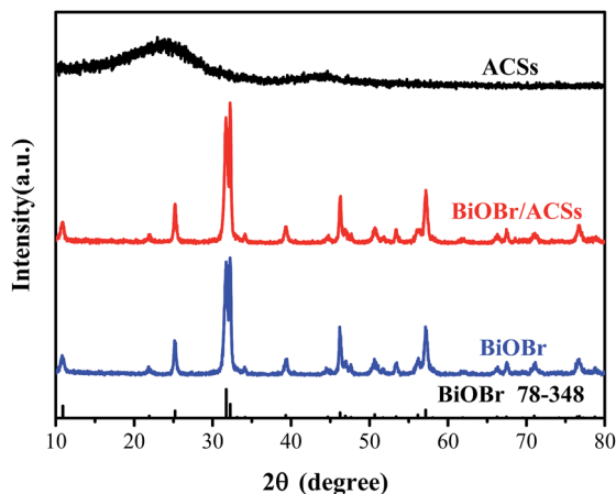
Fig. 1 XRD patterns of ACSs, BiOBr/ACSs and BiOBr samples.
