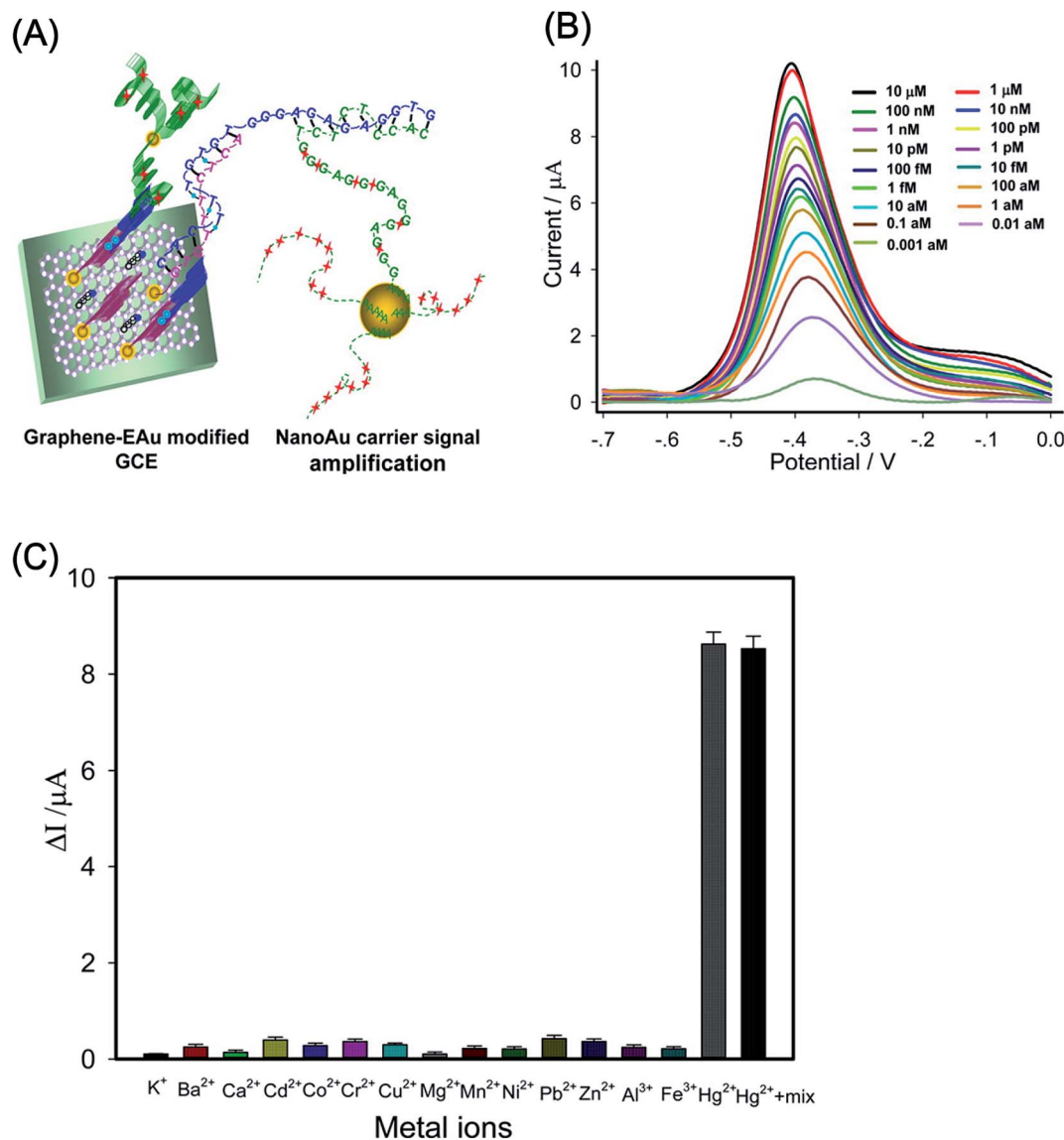
Fig. 28 (A) Schematic illustration of the sensing strategy for the detection of Hg 2+ using a graphene/nano-Au composite for signal amplification. (B) Square wave voltammograms (SWV) of mercuric biosensor as a function of Hg 2+ ions concentration in the 10 μM to 0.001 aM range in 20 mL Tris having 10 mM KCl. (C) Mercuric biosensor showing the selectivity of Hg 2+ ions among various interfering metal ions measured using 10 nM of Hg 2+ , 500 nM of interfering metal ions K + , Ba 2+ , Ca 2+ , Cd 2+ , Co 2+ , Cr 2+ , Cu 2+ , Mg 2+ , Mn 2+ , Ni 2+ , Pb 2+ , Zn 2+ , Al 3+ , Fe 3+ , and their corresponding mixture having 10 nM of Hg 2+ respectively. [Reprinted with permission from ref. 594, Y. Zhang, G. M. Zeng, L. Tang, J. Chen, Y. Zhu, X. X. He and Y. He, Electrochemical Sensor Based on Electrodeposited Graphene-Au Modified Electrode and NanoAu Carrier Amplified Signal Strategy for Attomolar Mercury Detection, Anal. Chem. , 2015, 87 , 989–996. Copyright© American Chemical Society.]
