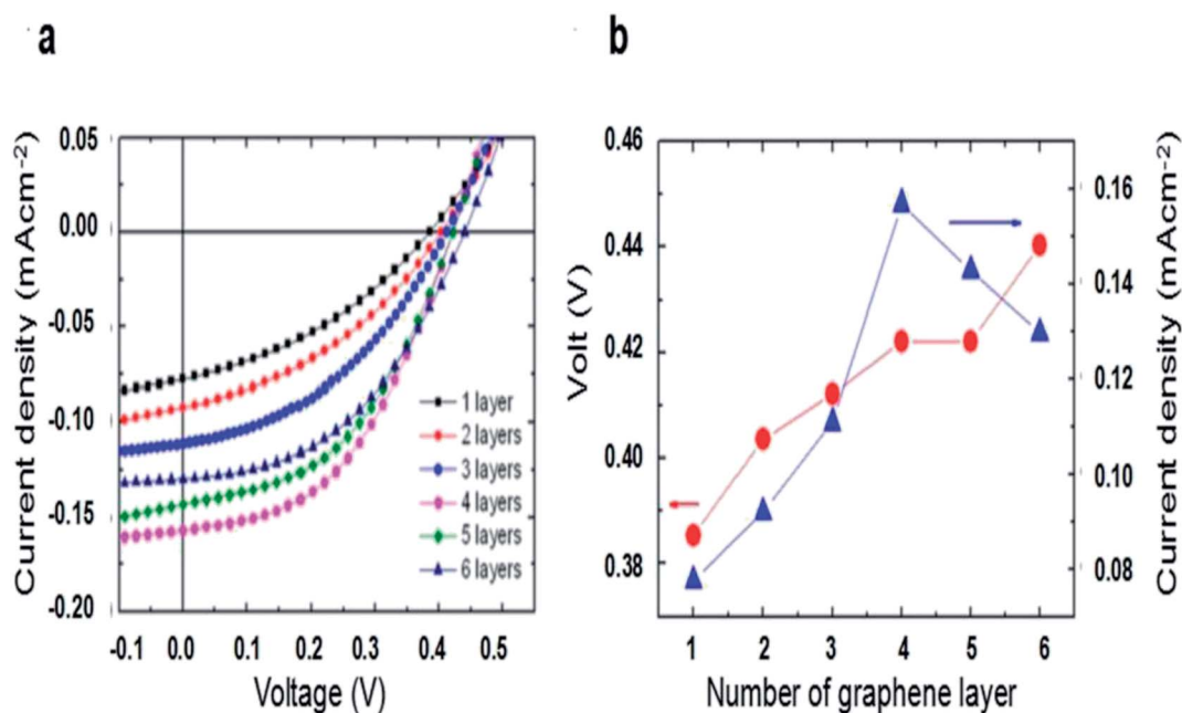
Fig. 5 (a) Current–voltage curves of solar cells based on graphene with 1, 2, 3, 4, 5, and 6 layers under illumination of 730 nm LED ( 2 mW cm^{-2} ). (b) The open-circuit voltage and short-circuit current of solar cells measured as functions of the number of graphene layers. (a and b) Reproduced from 51 with permission from American Institute of Physics.
