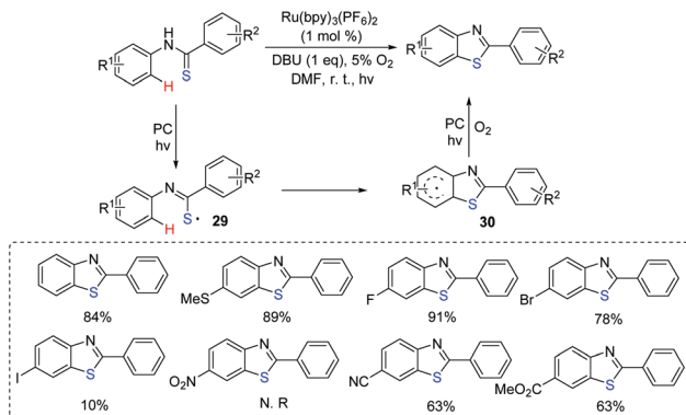
Scheme 14 Synthesis of 2-substituted benzothiazoles.
