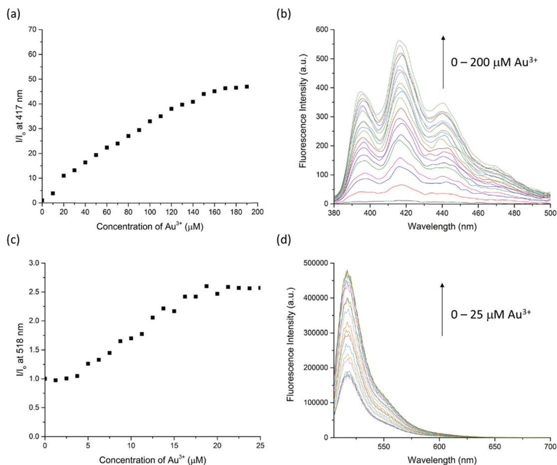
Fig. 6 (a) Fluorescence response of RRA ( 20 \mu\text{M} , \lambda_{\text{ex}} = 370 \text{ nm} ) at 417 \text{ nm} upon the addition of \text{Au}^{3+} ( 0-200 \mu\text{M} ) in THF/MeCN/ \text{H}_2\text{O} solution ( 2:48:50 , v/v/v). (b) Fluorescence spectral change of RRA ( 20 \mu\text{M} , \lambda_{\text{ex}} = 370 \text{ nm} ) at 417 \text{ nm} upon addition of \text{Au}^{3+} ( 0-200 \mu\text{M} ) in THF/MeCN/ \text{H}_2\text{O} solution ( 2:48:50 , v/v/v). (c) Fluorescence response of RRB ( 5 \mu\text{M} , \lambda_{\text{ex}} = 500 \text{ nm} ) at 518 \text{ nm} upon the addition of \text{Au}^{3+} ( 0-25 \mu\text{M} ) in MeCN/ \text{H}_2\text{O} solution ( 50:50 , v/v). (d) Fluorescence spectral change of RRB ( 5 \mu\text{M} , \lambda_{\text{ex}} = 500 \text{ nm} ) at 518 \text{ nm} upon addition of \text{Au}^{3+} ( 0-25 \mu\text{M} ) in MeCN/ \text{H}_2\text{O} solution ( 50:50 , v/v).
