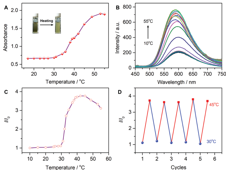
Fig. 5 LCST-featuring behavior: (A) temperature-dependent absorption at 430 nm of P(NIPAM-co-EM) (14 \mu\text{M} ) in an aqueous solution upon heating; inset: images of P(NIPAM-co-EM) before and after heating. (B) Temperature-dependent emission spectra of P(NIPAM-co-EM) (14 \mu\text{M} ), \lambda_{\text{ex}} = 430 nm. (C) The relative fluorescent intensity at 607 nm as a function of temperature. (D) Reversible thermo-response of P(NIPAM-co-EM) between 30 and 45 ^{\circ}\text{C} by monitoring the fluorescent signal.
