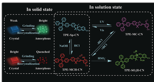
Scheme 1 Illustration of the switching states of TPE-Sp-CN with different stimuli.
