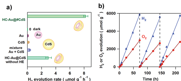
Fig. 5 (a) The comparison of the \text{H}_2 evolution rate for HC-Au( d_{\text{Au}} = 5.5 nm)@#CdS(I/CdS = 1.9 nm), Au colloid, CdS, and a mixture of Au and CdS under red-light illumination ( \lambda_{\text{ex}} = 640 nm) or dark conditions. (b) Repeated water splitting by HC-Au( d_{\text{Au}} = 12.1 nm)@#CdS(I/CdS = 2.1 nm) under red-light illumination. Figures are taken from ref. 59.
