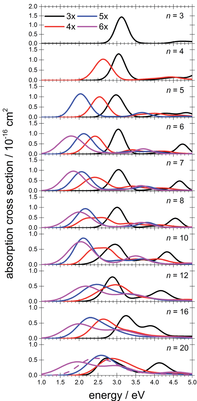
Fig. 2 Calculated spectra of selected [\text{Mg}(\text{H}_2\text{O})_n]^+ ions with different Mg coordination numbers ( 3\times - 6\times ). Calculated at the CAM-B3LYP/aug-cc-pVDZ// \omega B97XD/def2TZVP level of theory using the linearized reflection principle to calculate the peak width. Surface and inner isomers for n = 20 are shown with full and dashed lines, respectively. Benchmarking with respect to the ADC(2) method can be found in Fig. S4.†
