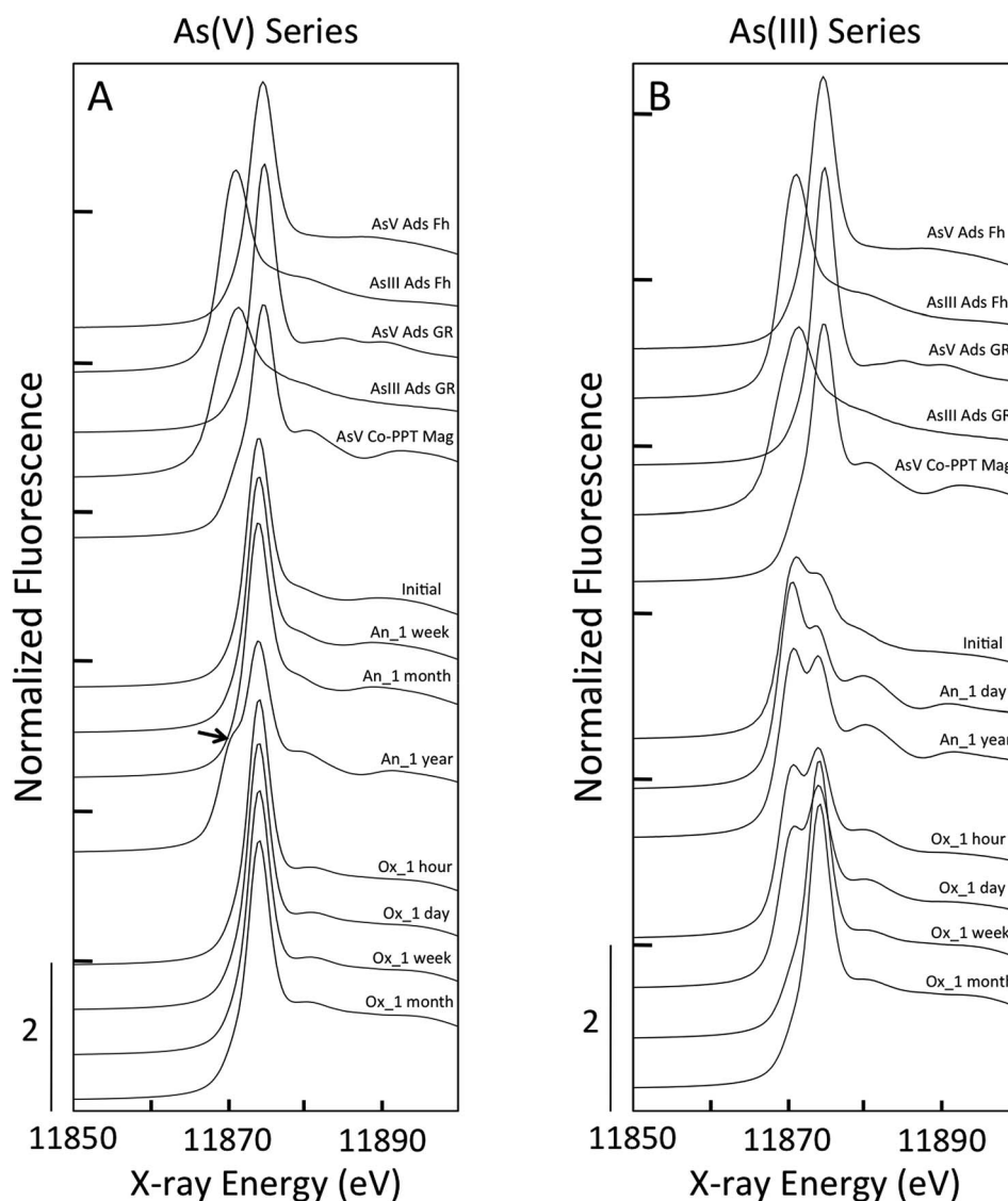
Fig. 5 As K-edge XANES spectra for green rust aging samples in As(v) experiments (A) and As(III) experiments (B). The experimental data are given below As(III) and As(v) bearing reference materials. The anoxic aging series (e.g. An_1 week) are given above the oxic aging samples (e.g. Ox_1 hour). The arrow in A highlights a shoulder in the anoxic aging sample resulting from the presence of As(III).
