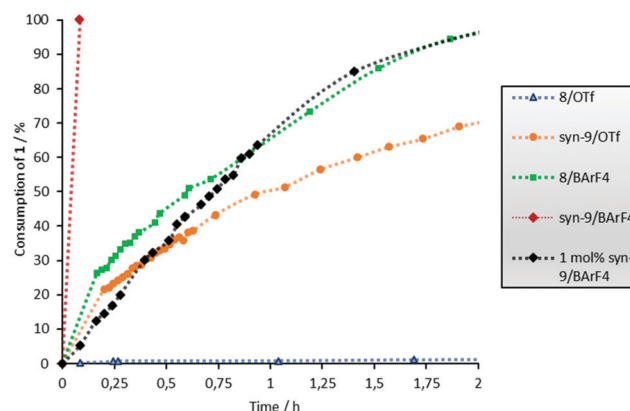
Fig. 2 Consumption of 1 versus the time profile of the Nazarov cyclisation with 5 mol% catalyst (unless noted otherwise) and c 0 ( 1 ) = 15.4 mM. No reaction without a catalyst and with compounds 3–7 and 11–13 . The error is approximately 5%.
