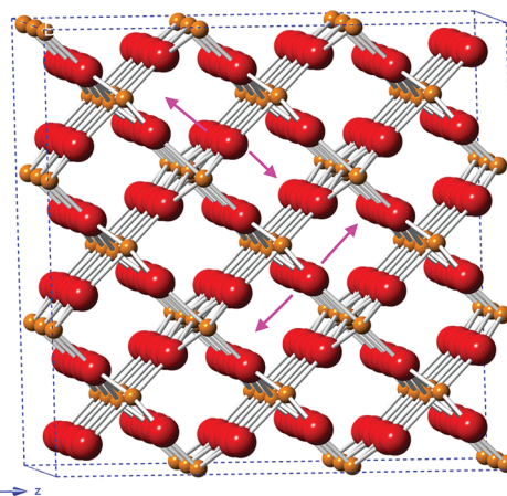
Fig. 8 Structure of monoclinic VO 2 , based on ICSD 34033, indicating the direction of the proposed out-of-plane oxygen displacement (purple arrows). O 2- : red; V 4+ : orange.
