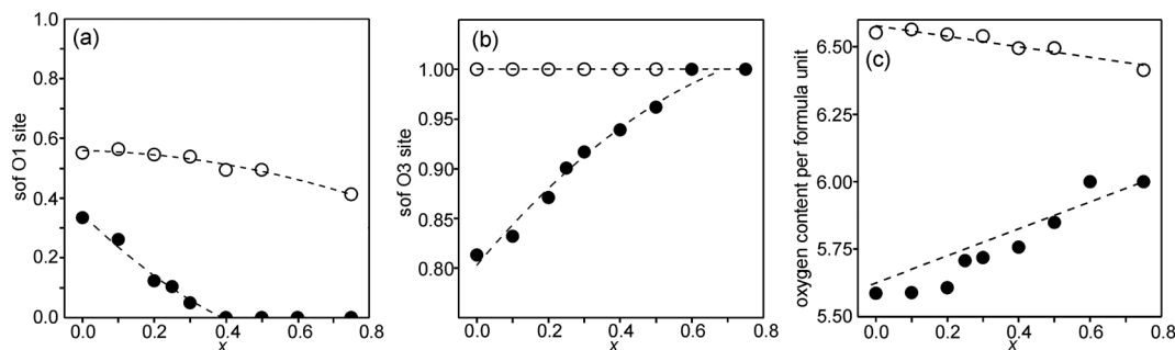
Fig. 4 Refined softs from NPD data for (a) the O1 site, (b) the O3 site, and (c) the derived total O content per formula unit. Filled circles denote the as-prepared samples and open circles denote the air-annealed samples. The sof for O3 was for the air-annealed samples set to one for all x as well as for the as-prepared samples for x \geq 0.6 . The sof for O1 was for the as-prepared samples set to zero for x \geq 0.4 . The dashed lines are for eye guidance only, except for the O content of the as-prepared samples, which shows the expected O content of nominal compositions with only \text{Fe}^{3+} and \text{Ni}^{2+} ions.
