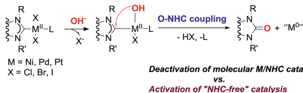
Scheme 1 Discovered O–NHC coupling reactions in M/NHC systems.
