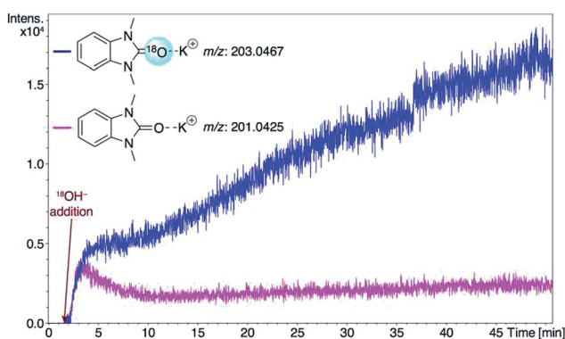
Fig. 2 Real-time abundances of 7a -[ ^{18}\text{O} ] and 7a -[ ^{16}\text{O} ] (in ionic [\text{M} + \text{K}]^+ form) in the reaction between complex 2a and \text{K}^{18}\text{OH}_{\text{aq}} in THF at 100^\circ\text{C} . Solution of KOH in \text{H}_2^{18}\text{O} was added after 1.2 min of recording.
