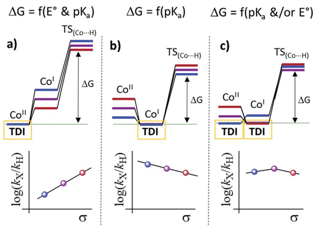
Fig. 12 Simplified mechanism scenarios from the Co II species to the Co I protonation transition state and related Hammett plots considering the electronic effects in hypothetical situations regarding the reducing redox potentials of PS n/n-1 (photosensitizer) and Co II/I couples. (a) E_{1/2}(\text{Co}^{\text{II/I}}) value is substantially more reducing than E(\text{PS}^{\text{n/n-1}}) , (b) E(\text{PS}^{\text{n/n-1}}) value is substantially more reducing than E_{1/2}(\text{Co}^{\text{II/I}}) , (c) E(\text{PS}^{\text{n/n-1}}) value is intermediate in the E_{1/2}(\text{Co}^{\text{II/I}}) series.
