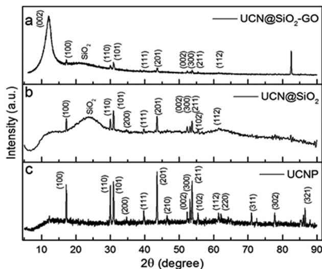
Fig. 5 XRD spectra of UCNP, UCN@SiO 2 NPs and UCN@SiO 2 -GO nanocomposite.
