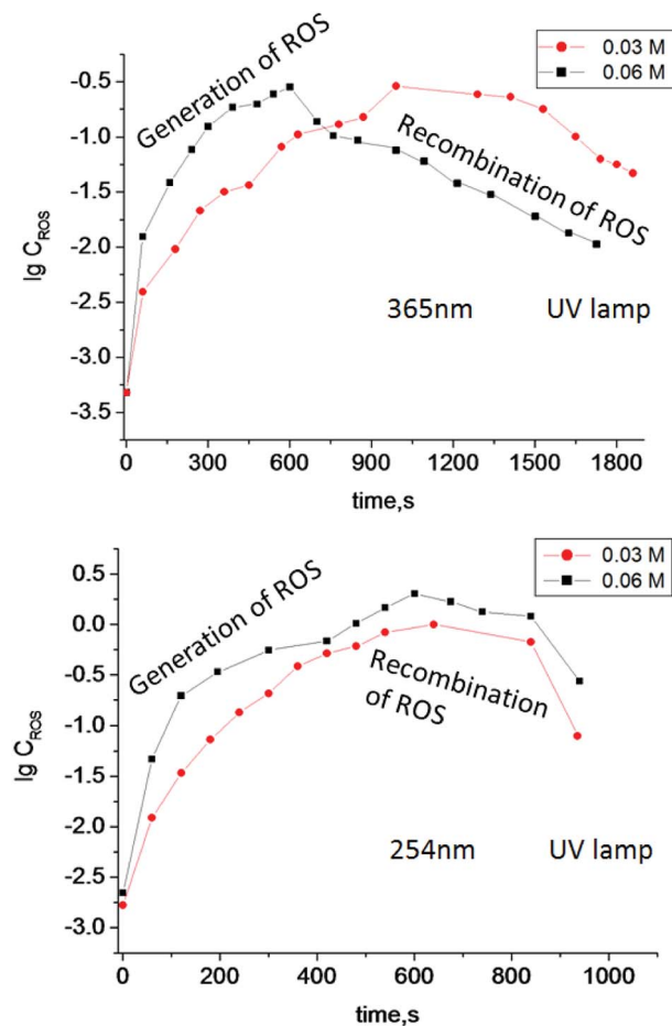
Fig. 3 Log concentration of ROS generated in TiO 2 suspensions of different concentration (0.03 M and 0.06 M) under irradiation by UV light with different wavelengths vs. irradiation time.
