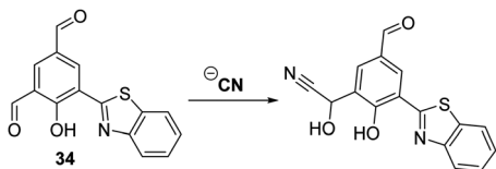
Scheme 32 A selective HBT fluorescent probe 34 for the detection of \text{CN}^- . Measurement conditions: ACN only.
