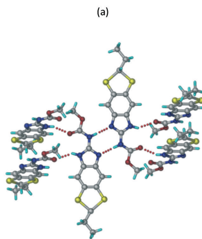
Fig. 1 ABZ crystal structures reported in the literature. ABZ exhibits sulphur attached alkyl disorder and the imidazole rings show tautomerism labelled as (a) form II (ref. 9) and (b) form I. 10 CSD ref codes SUTWIO, BOGFUZ.
