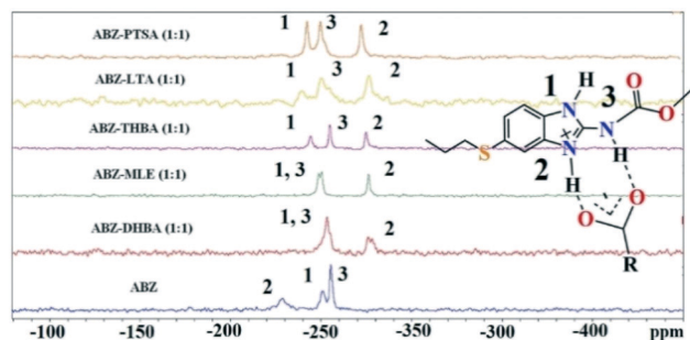
Fig. 9 ^{15}\text{N} ss-NMR of the ABZ salts.
