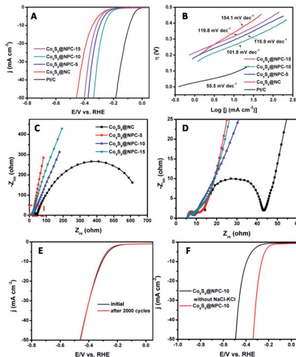
Fig. 4 (A) HER polarization curves for Co 9 S 8 @NPC-5, Co 9 S 8 @NPC-10, Co 9 S 8 @NPC-15, Co 9 S 8 @NPC-10, Co 9 S 8 @NPC-15, Co 9 S 8 @NC and Pt/C at 5.0 mV s -1 in 1.0 M KOH. (B) Corresponding Tafel plots for Co 9 S 8 @NPC-5, Co 9 S 8 @NPC-10, Co 9 S 8 @NPC-15, Co 9 S 8 @NC and Pt/C. (C and D) EIS Nyquist curves for Co 9 S 8 @NPC-5, Co 9 S 8 @NPC-10, Co 9 S 8 @NPC-15 and Co 9 S 8 @NC obtained by applying a sine wave with an amplitude of 5.0 mV over the frequency range from 10 -1 to 10 6 Hz, where the enclosed area of (C) is magnified in (D). (E) LSV curves for Co 9 S 8 @NPC-10 before and after 2000 CV cycles from -0.3 to +0.2 V at 50 mV s -1 . (F) HER polarization curves for electrodes of Co 9 S 8 @NPC-10 and Co 9 S 8 @NPC-10 without NaCl-KCl at a scan rate of 5.0 mV s -1 in 1.0 M KOH.
