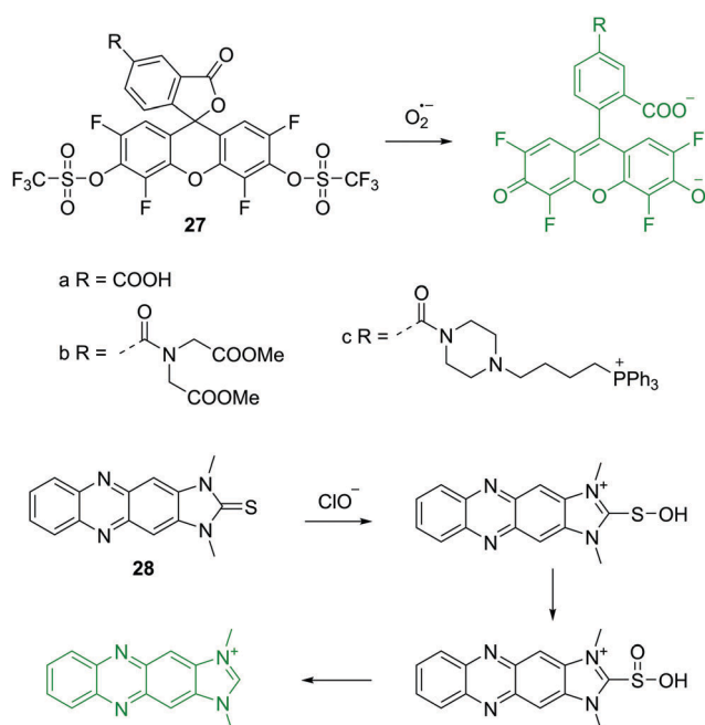
Fig. 13 Structures and proposed mechanism of 27 and 28 for detection of O_2^{\cdot-} and ClO^- respectively.
