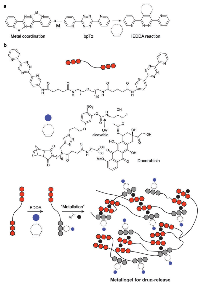
Fig. 59 Synthesis of metallo-hydrogels. (a) Diels–Alder reaction and metal coordination of bpTz. (b) Representation of the drug release approach triggered by photo decaging from the metallo-hydrogel.
