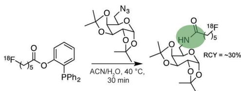
Fig. 41 (a) Click methods for radiosynthesis. (i) CuAAC click reaction for preparation of radiotracers including the synthesis of the most common prosthetic groups. (ii) ^{99\text{m}}\text{Tc(CO)}_3(\text{H}_2\text{O})_3^{3+} radiolabelling through complexation by triazole moieties formed by CuAAC cycloaddition. (b) Copper-free click radiolabelling by SPAAC reaction. (i) ^{18}\text{F} introduced into the cyclooctyne prosthetic group ( ^{18}\text{F} -labelled aza-dibenzocyclooctyne derivative, [ ^{18}\text{F} ]-ADIBO) and then subjected to strain-promoted cyclization with azide-functionalized biomolecules. 248 (ii) Labelling of ADIBO-functionalized biomolecules with ^{18}\text{F} -azides. 249 (c) Staudinger radiolabelling. 257 (d) Other examples of click radiolabelling. (i) Radiolabelling by oxime formation between an aminoxy-functionalized peptide and a ^{18}\text{F} -fluorobenzaldehyde ([ ^{18}\text{F} ]FBA). (ii) Cyanobenzothiazole–cysteine (CBT–Cys) condensation reaction for ^{18}\text{F} -radiolabelling.
