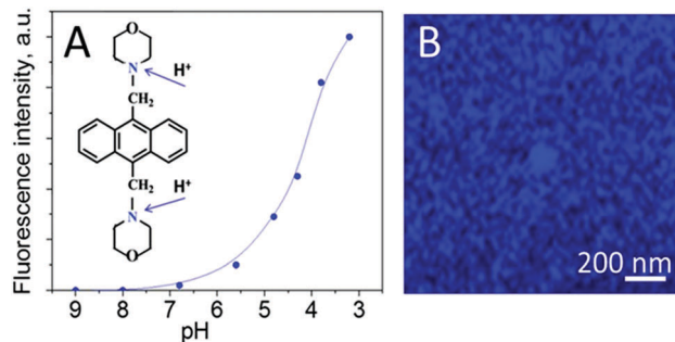
Fig. 3 (A) Calibration of fluorescent pH indicator, 4,4'-(anthracene-9,10-diyl(dimethanediy))dimorpholine, that exhibits a pK_a \sim 5.1 , and initial chemical formula showing the protonation sites; (B) confocal fluorescent images of the TiO_2 surface immediately after irradiation.
