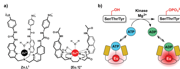
Fig. 1 (a) Structures of complexes \text{Zn}(\mathbf{L}1) and [\text{Eu}(\mathbf{1})]^+ ; (b) cartoon illustrating continuous monitoring of kinase activity using [\text{Eu}(\mathbf{1})]^+ . The \text{Eu}(\text{III}) complex binds reversibly to ATP and ADP, providing a ratiometric luminescent signal that precisely indicates the ADP/ATP ratio.
