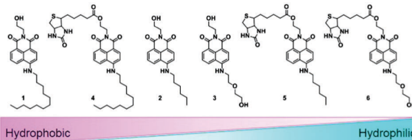
Fig. 2 Lipophilicity of probes ( 1–6 ) according to \log P_{\text{oct}} value.
