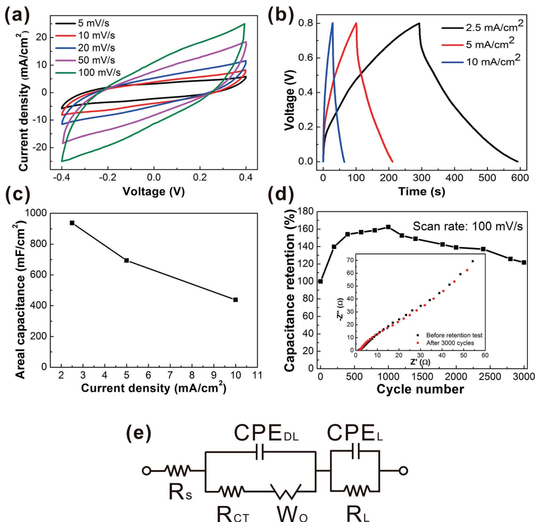
Fig. 3 CV (a) and GCD (b) curves of the C-web@Ni-cotton supercapacitor fabric tested in 1 M Na 2 SO 4 liquid electrolyte. (c) Summary of the areal capacitance of the supercapacitor at different current densities. (d) Retention performance of supercapacitor (scan rate: 100 mV s -1 ). The inset graph shows the change of EIS spectra before and after cyclic performance testing. (e) The equivalent circuit of the C-web@Ni-cotton supercapacitor fabric, where R_s is the equivalent series resistance (ESR), R_{ct} is the resistance of the electrode-electrolyte (charge transfer resistance), R_l is the leakage resistance, CPE_{DL} is the electrical double layer capacitance, W_o is the Warburg element, and CPE_L is the pseudocapacitance.
