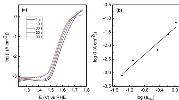
Fig. 7 (a) Tafel plots showing OER performance for Au/ \text{Co}(\text{OH})_2 electrodeposited from 10\text{ mM Co}(\text{NO}_3)_2 \cdot 6\text{H}_2\text{O} at different deposition time, (b) effect of hydroxide ion activity on OER. The cyclic voltammetric experiments used to obtain the data was recorded at a sweep rate of 1\text{ mV s}^{-1} in 1\text{ M NaOH} .
