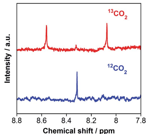
Fig. 3 ^1\text{H} NMR spectra of the aqueous reaction solutions (1 mL) containing RuRu /Ag/TaON (4 mg) and EDTA·2Na (10 mM), measured after 24 h irradiation at \lambda_{\text{ex}} > 400 nm under ^{13}\text{CO}_2 (red) and ^{12}\text{CO}_2 (blue) atmospheres.
