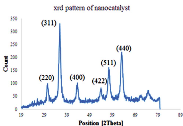
Fig. 3 The X-ray diffraction pattern of Cu(II) immobilized on \text{Fe}_3\text{O}_4@SiO_2@L\text{-arginine} nanoparticle.
