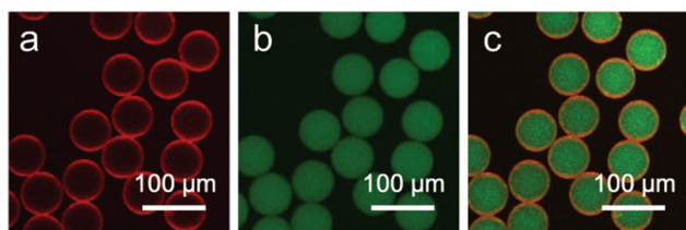
Fig. 5 CLSM images of microdroplets encapsulating fluorescein iso-thiocyanate-dextran cargo and capsule-forming components: MCP, AP and CB[8]. (a) Red channel: Rhodamine B-labelled AP, (b) green channel: FD and (c) overlaid.
