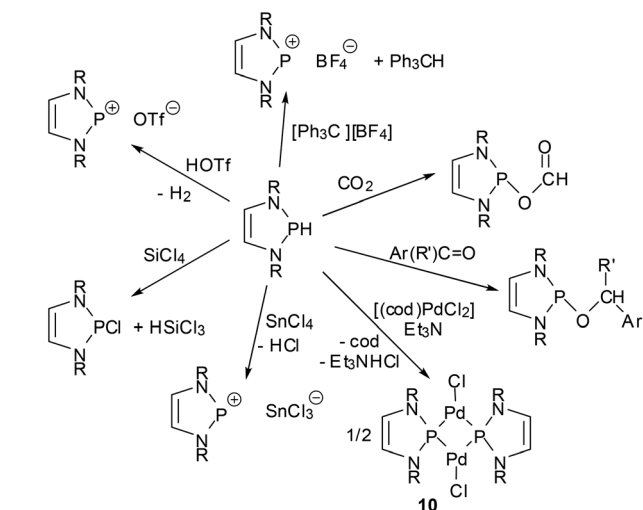
Scheme 10 Selected stoichiometric reactions of P-hydrogen DAPs (R = alkyl, aryl; R' = aryl, H; cod = 1,5-cyclooctadiene).
