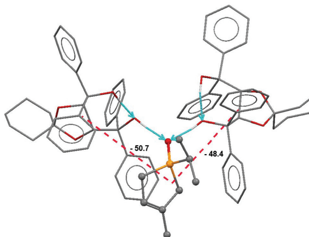
Fig. 5 The two largest attractive interactions (in kJ mol -1 ) indicated also by red broken lines between the respective molecular centres in the crystal of the ( S )-( - )-1-isopropyl-3-methyl-3-phospholene oxide guest [( S ) -1g ] with two independent spiro-TADDOL [( - ) 10 ] hosts. Arrows indicate the donor–acceptor directions of the H-bond vectors.
