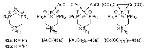
Fig. 7 Zwitterionic triphosphenium derivatives 43a,b (a: R = Ph, b: R = i Pr) and selected coordination complexes with AuCl and [Co(CO) 3 ].
