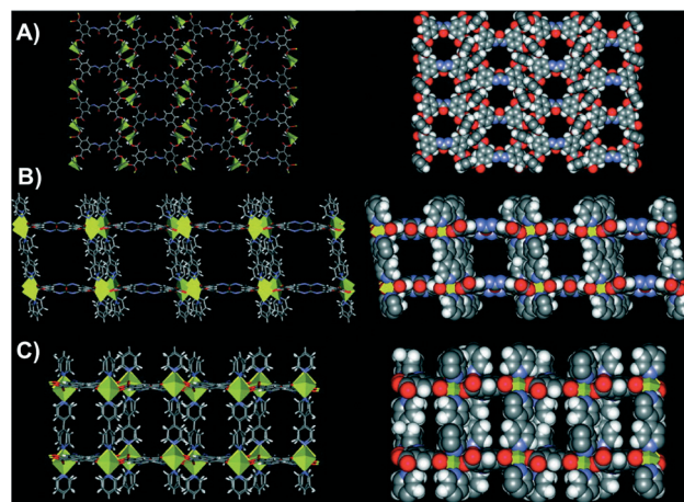
Fig. 2 Stick and space-filling representations of NU-601 (P 2 1 /c space group). A) View down the a axis (pore size 12.05 Å × 13.95 Å). B) View down the b axis (pore size 11.38 Å × 13.69 Å). C) View down the c axis (pore size 11.38 Å × 4.87 Å). Adapted with permission from ref. 43. Copyright © American Chemical Society.
