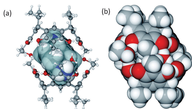
Fig. 2 Dimeric capsule, (\text{TDAC})^{2+}@[1\text{-H}_2\text{O-MeOH}]_2 shown in (a) as ball and stick with the calculated cavity in transparent grey colour and the guest (\text{TDAC})^{2+} as CPK to illustrate the very tight encapsulation and (b) as the CPK model.
