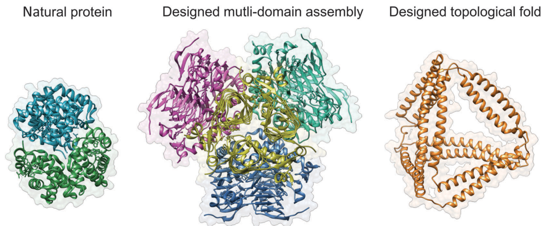
Fig. 1 Protein design strategies. Haemoglobin (PDB ID 2DN2) is shown as a typical representative of natural globular proteins. The designed multi-domain assembly (PDB ID 4EGG) is composed of four trimeric subunits, with their contact interfaces carefully designed to produce a symmetric tetrahedral structure. The result is a large, bulky assembly with a solid core, similar in principle to most natural proteins. Designed topological protein composed of concatenated coiled-coil dimer forming modules yields a tetrahedral protein cage with a large cavity in the centre (structural model taken from ref. 24). Images were created with UCSF Chimera. 61
