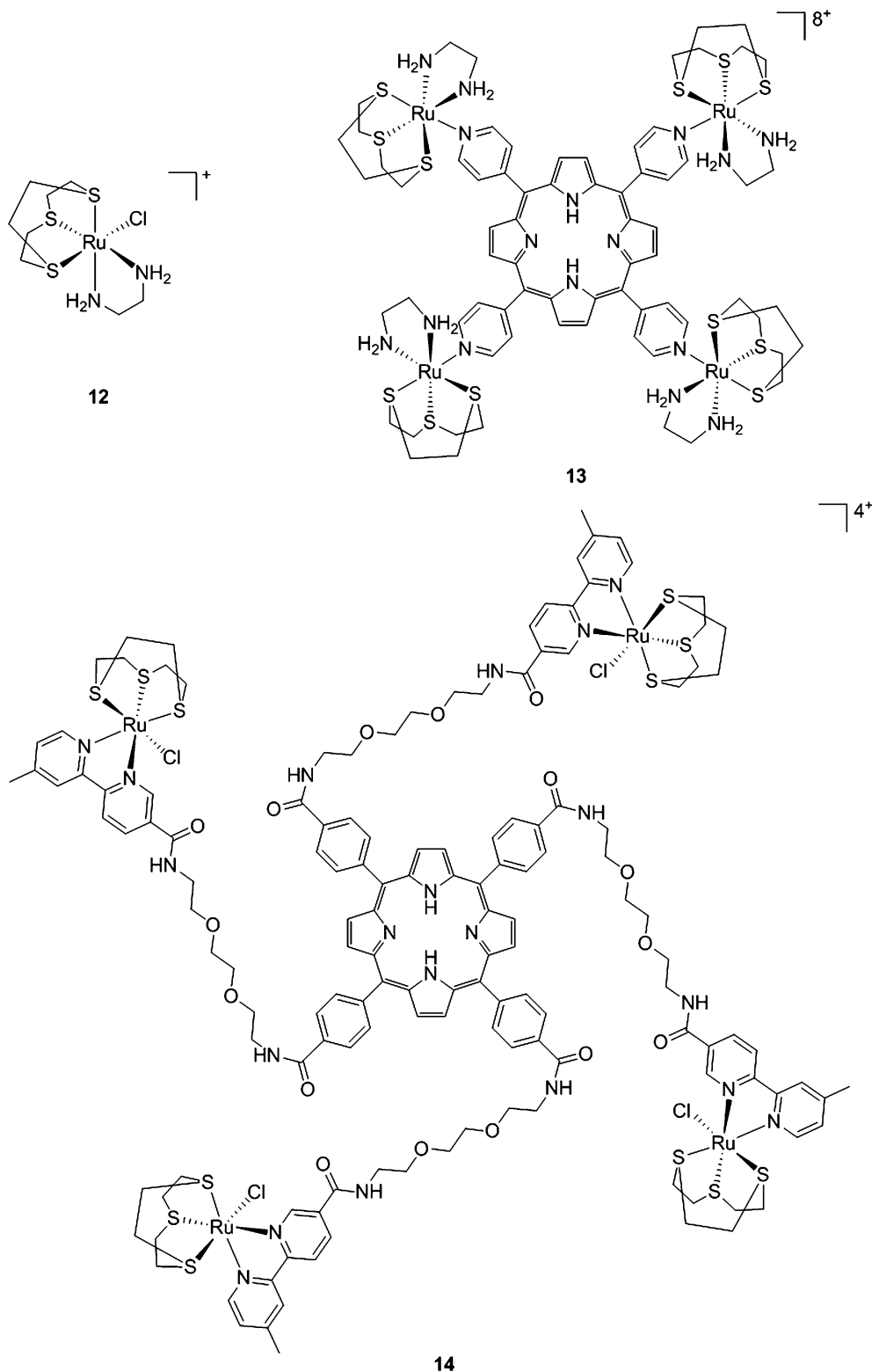
Fig. 11 Structures of \text{Ru}(\text{[9]aneS}_3)(\text{en})\text{Cl}]^+ (top, left) and of the ruthenium-derivatized porphyrin systems 13 and 14 . 40
